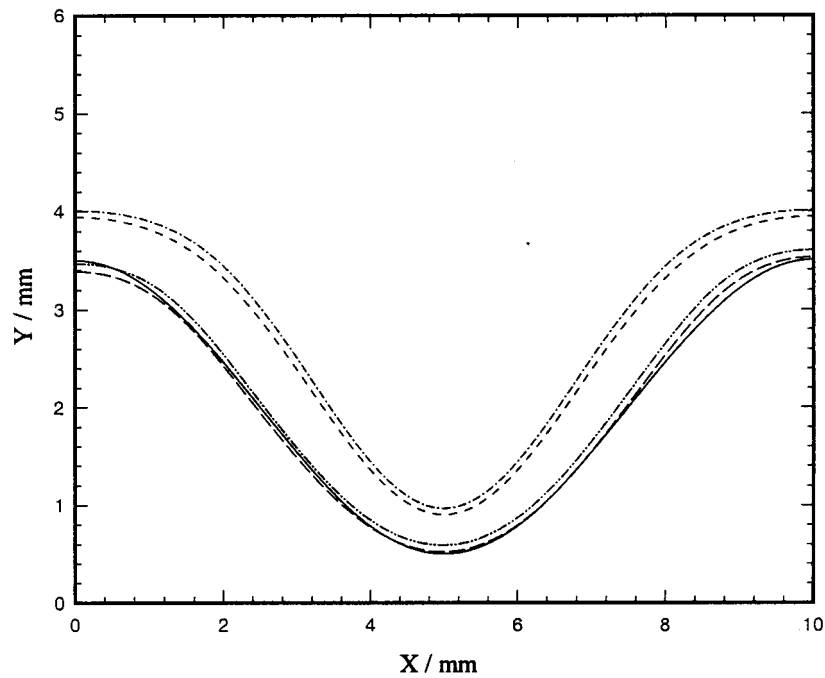
Fig. 8. Predicted tool shapes with/without the flow effect and the corresponding workpiece shapes. Desired workpiece shape is r(x) = 2 + 1.5 \cos(\pi x/5) . Key: (-----) tool shape neglecting flow effect (tool1); (- . - . -) tool shape considering flow effect (tool2); (.....) workpiece shape obtained from tool1; (---) workpiece shape obtained from tool2; (—) desired workpiece shape.
