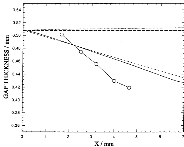
Fig. 2. Comparisons of workpiece shape between numerical and experimental results. Key: (O) experimental data [21]; (---) Hopfenfeld and Cole; (-.-.-) neglect flow effects model; (—) one-dimensional two-phase model; (.....) two-dimensional single-phase model.
