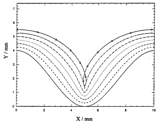
Fig. 7. Desired workpiece shape ( \beta = 2 ) and tool shapes predicted by different values of \phi_a/f_r : (— \Delta —) 6709.02, (-----) 5590.85, (---) 4472.68, (—) 3354.51, (-----) 2236.34 and (- - - - -) 1118.17 \text{ V mm}^{-1} \text{ s} ; (—) desired workpiece.
