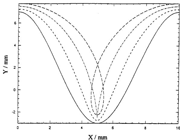
Fig. 6. Desired workpiece shape ( \beta = 5 ) and tool shapes predicted by different values of \phi_a/f_r : (---) 3354.51, (-----) 2236.34 and (- - - - -) 1118.17 \text{ V mm}^{-1} \text{ s} ; (—) desired workpiece.
