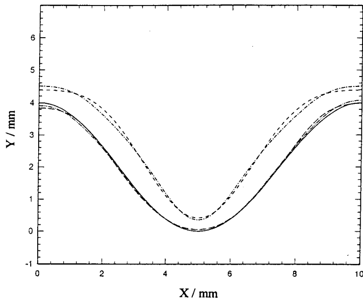
Fig. 10. Predicted tool shapes and corresponding workpiece shapes for various degrees of m in Fourier series. Desired workpiece shape is r(x) = 2 + 2.0 \cos(\pi x/5) . Key: (- - - -) tool shape ( m = 3 ); (- · - · -) tool shape ( m = 5 ); (- - -) workpiece shape ( m = 3 ); (· · · · ·) workpiece shape ( m = 5 ); (—) desired workpiece shape.
